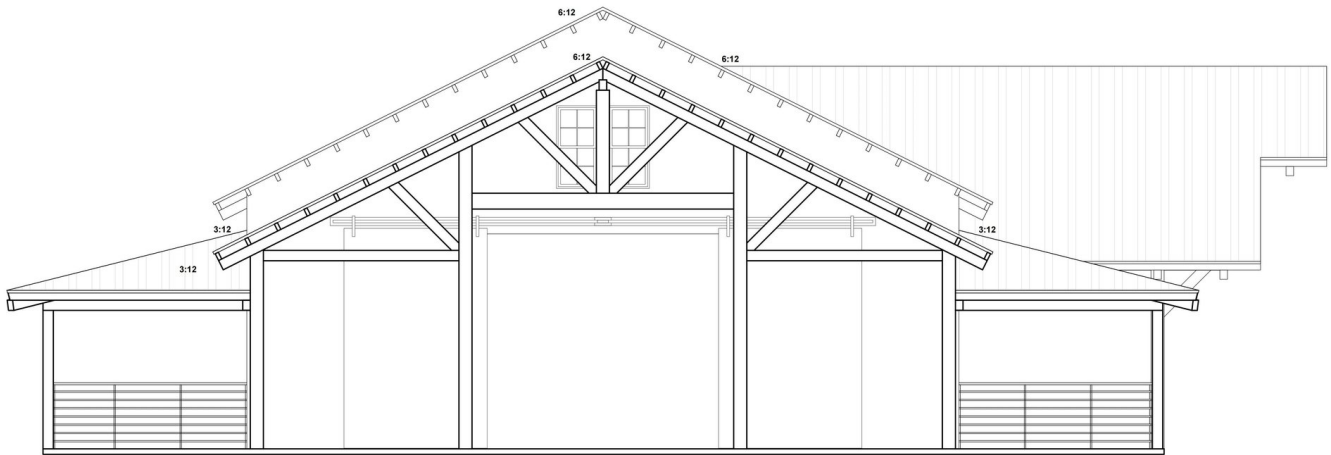
LEFT ELEVATION
