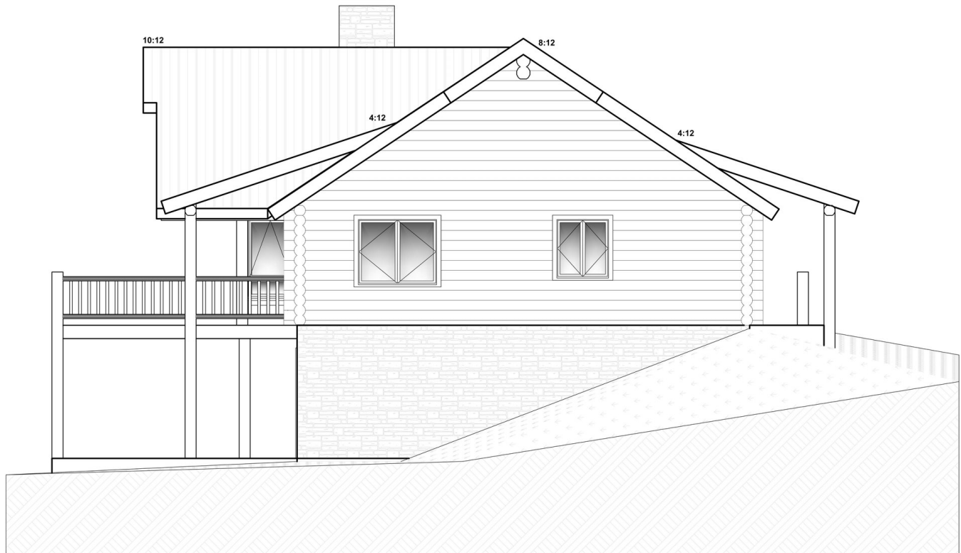
LEFT ELEVATION
