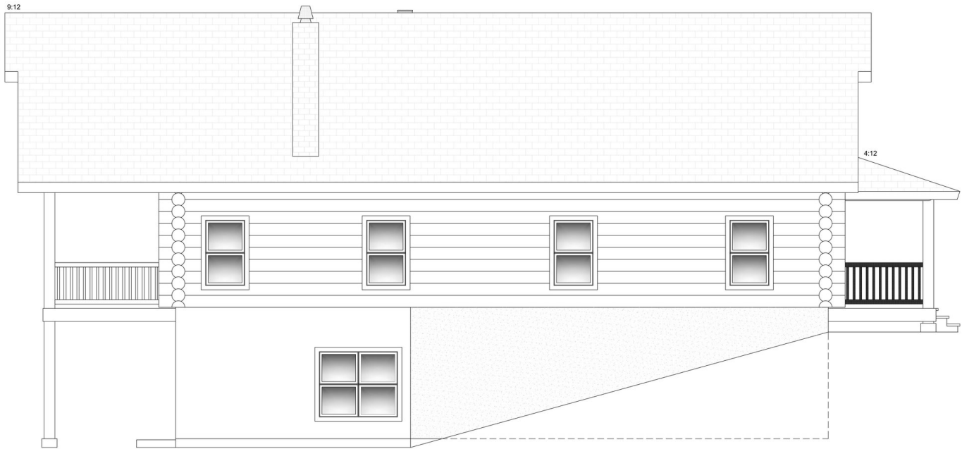
LEFT ELEVATION
