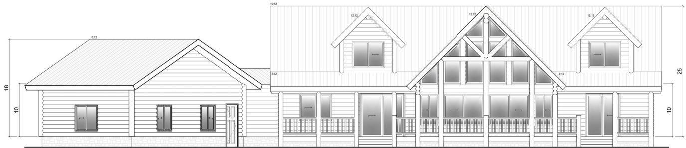
FRONT ELEVATION
