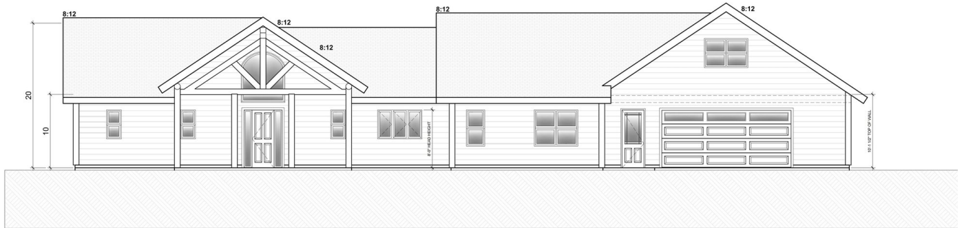
FRONT ELEVATION
