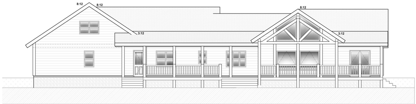
REAR ELEVATION
