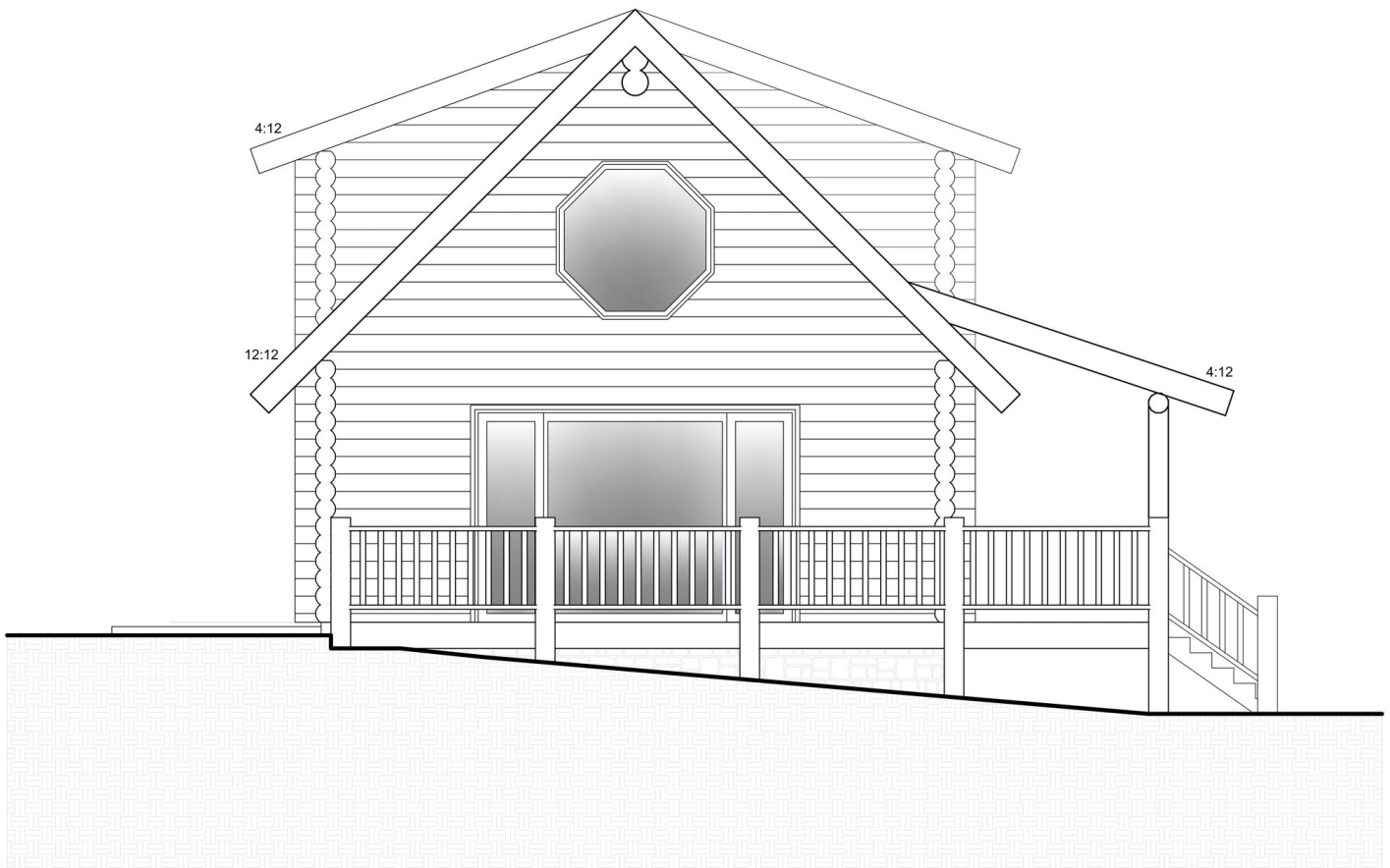
LEFT ELEVATION
