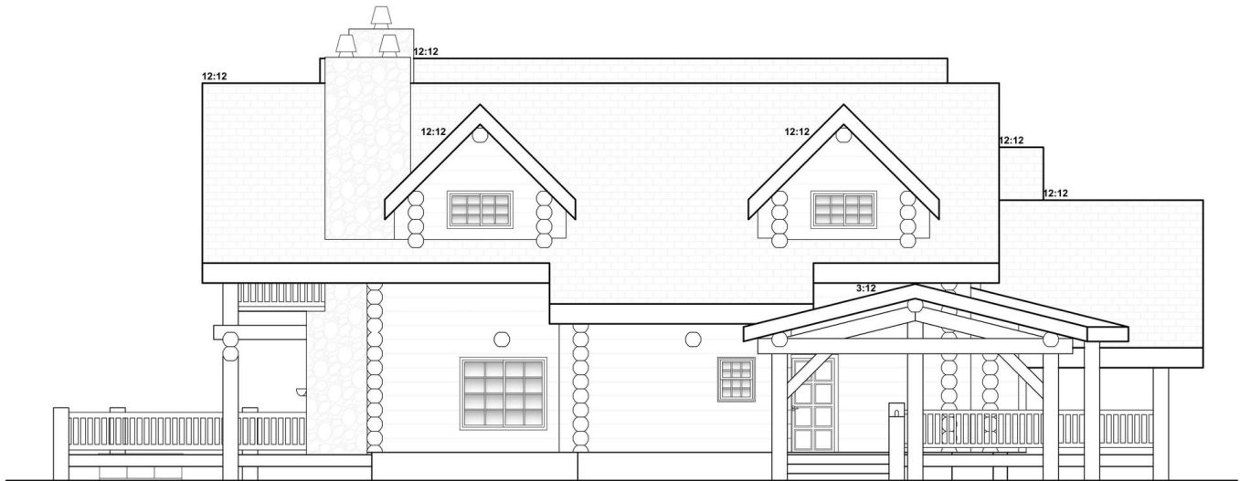
LEFT ELEVATION
