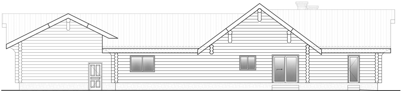
REAR ELEVATION
