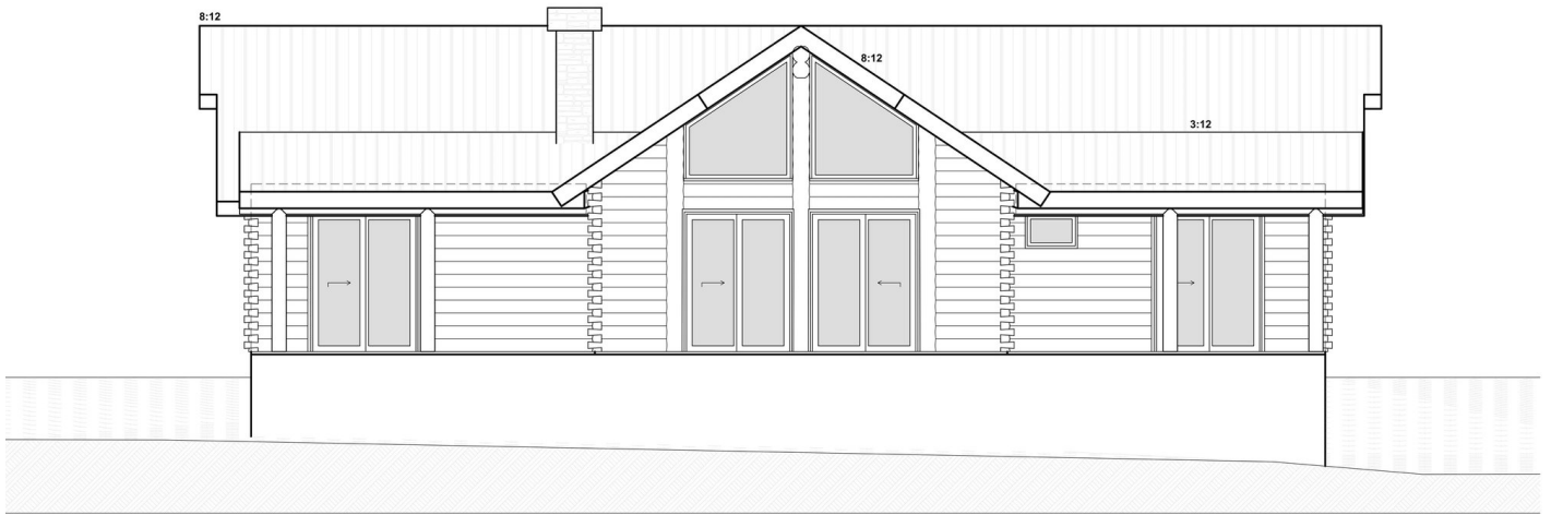
REAR ELEVATION
