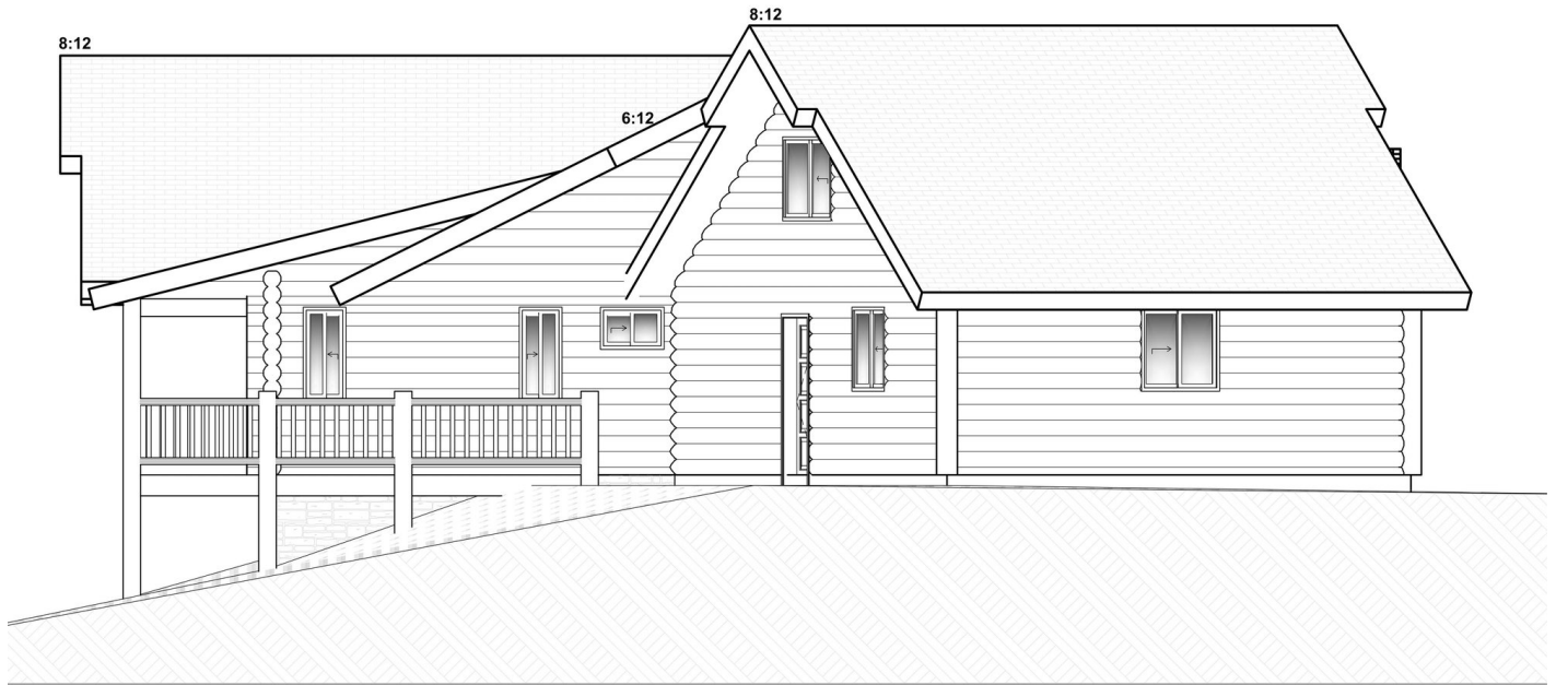
LEFT ELEVATION
