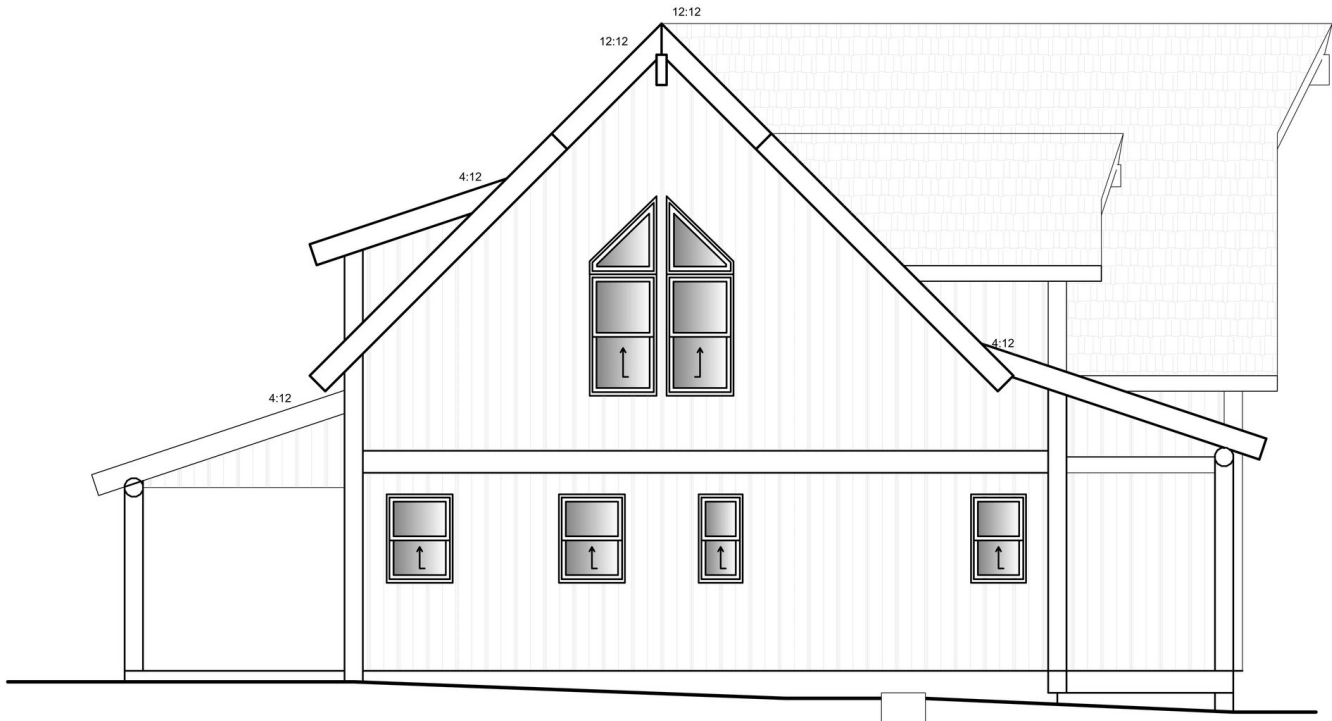
LEFT ELEVATION
