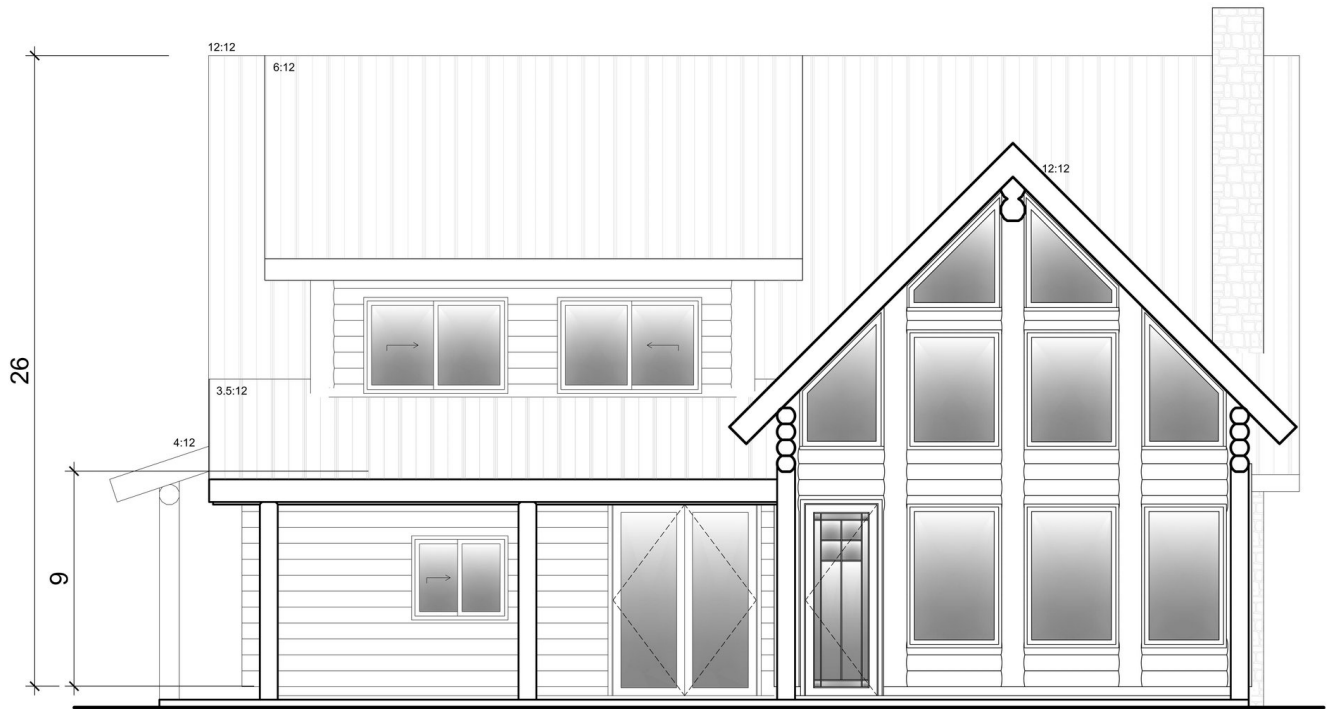
FRONT ELEVATION
