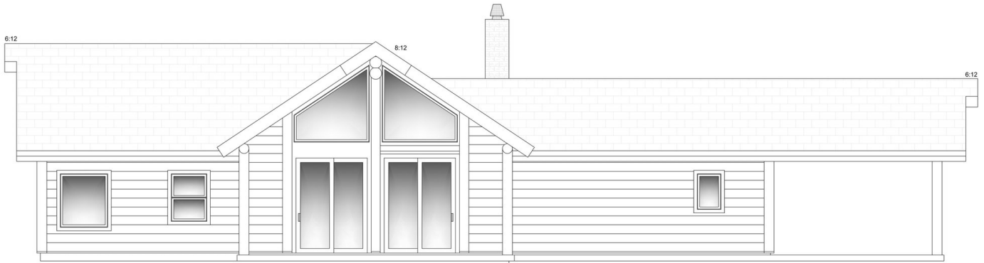
LEFT ELEVATION
