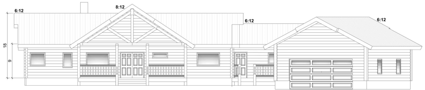
FRONT ELEVATION
