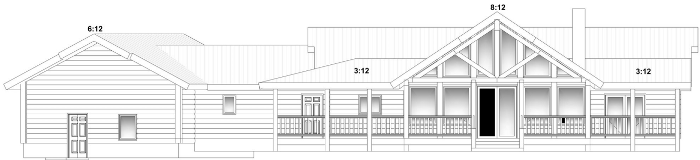
REAR ELEVATION
