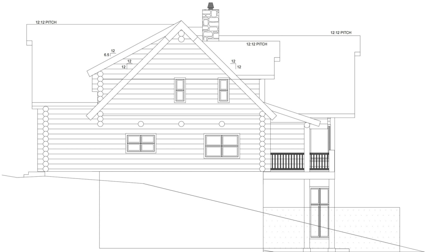
LEFT ELEVATION
