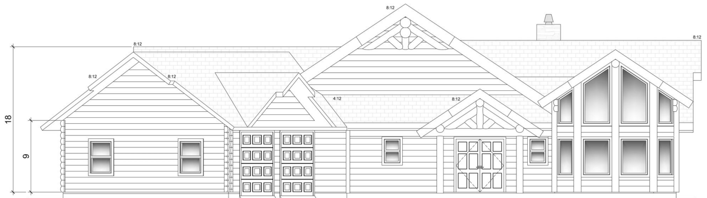
FRONT ELEVATION
