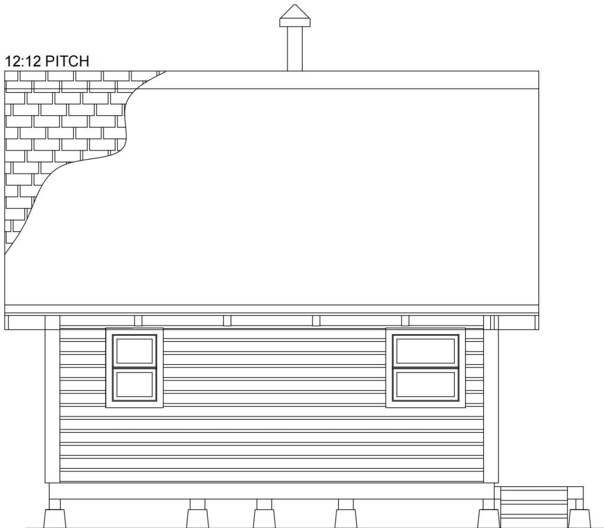
LEFT ELEVATION
