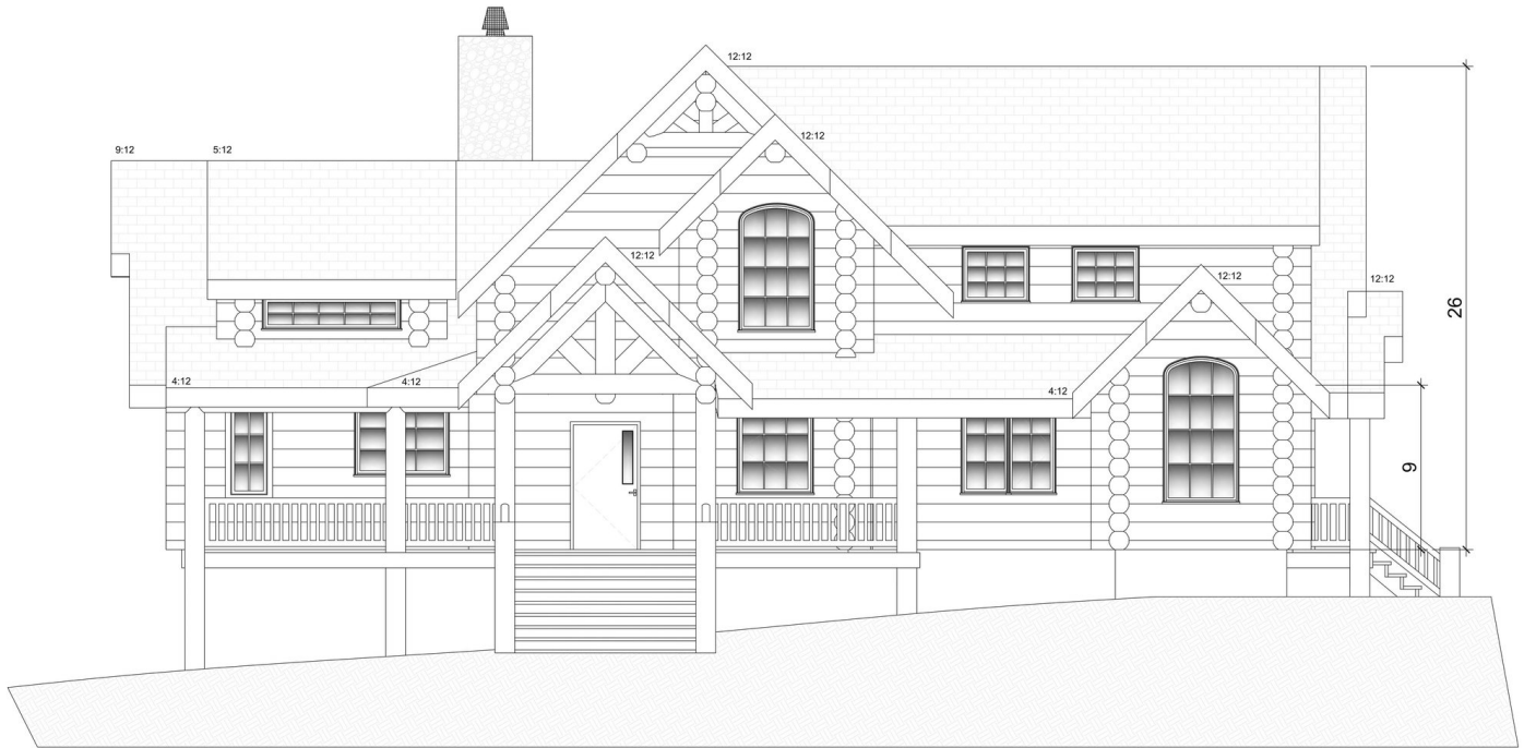
FRONT ELEVATION
