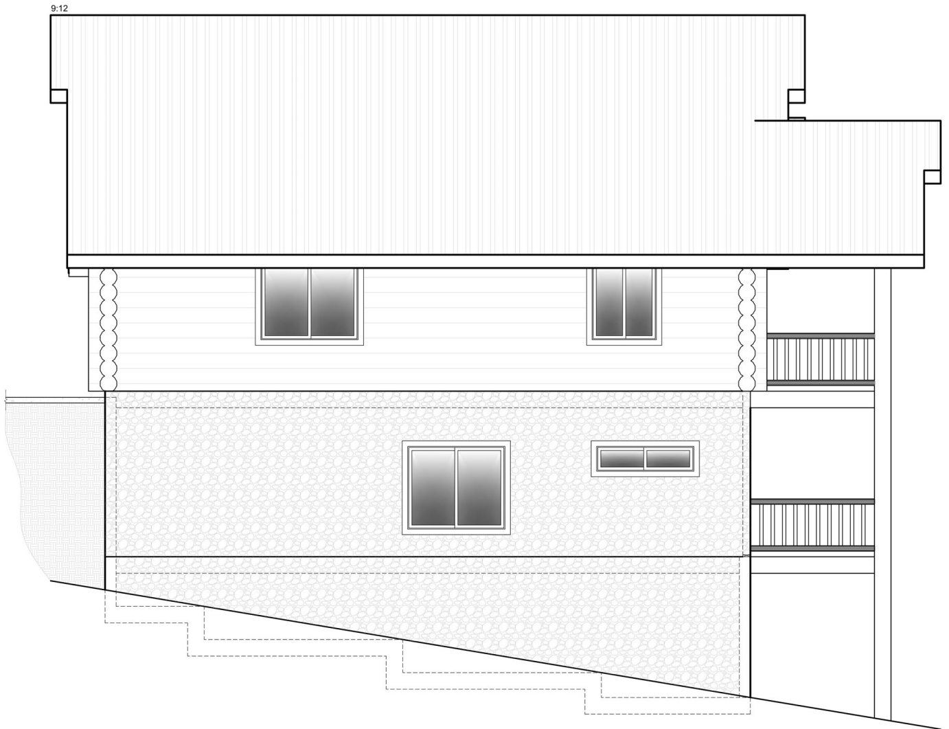
LEFT ELEVATION
