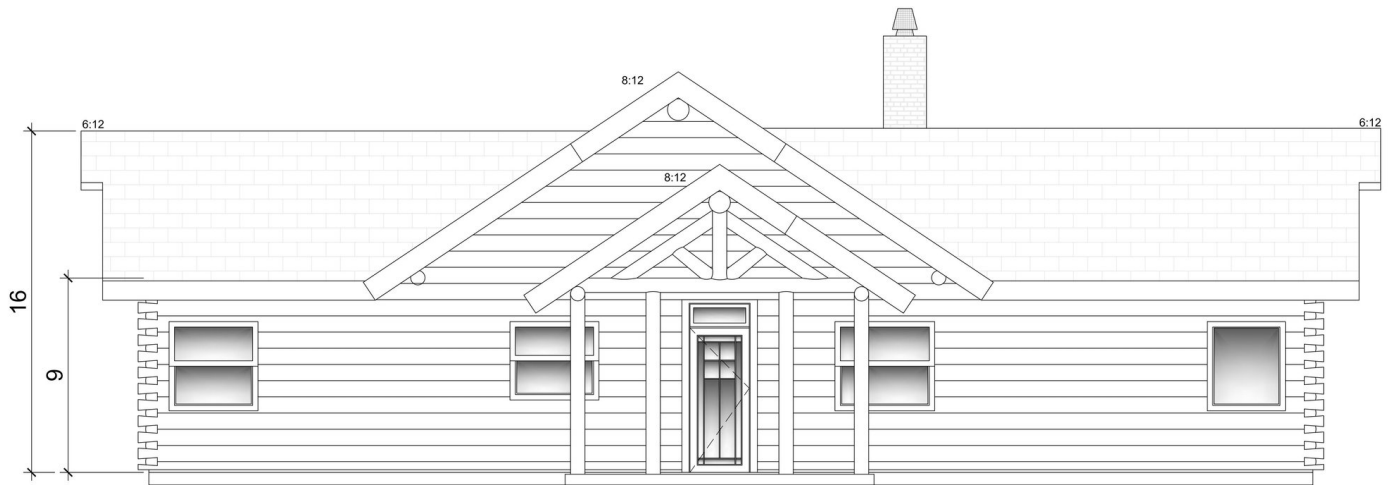
FRONT ELEVATION
