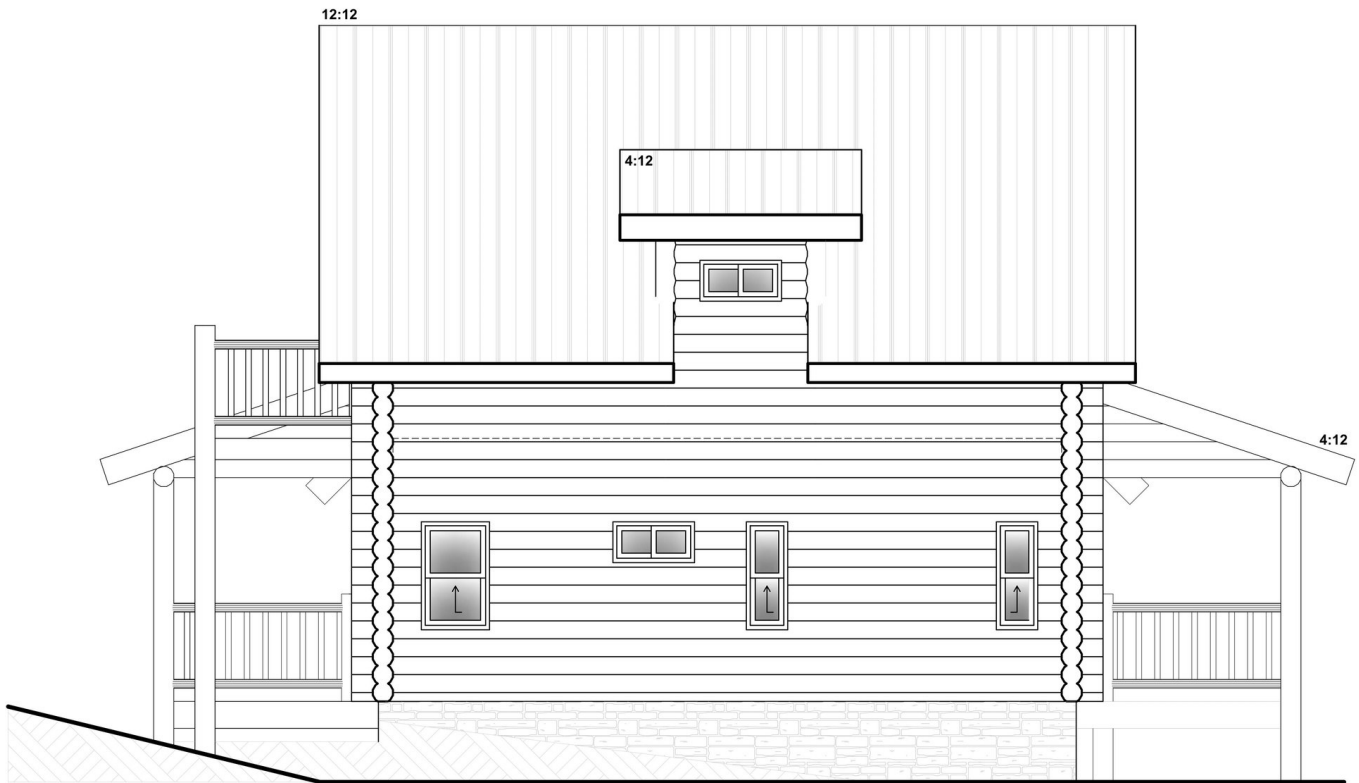
LEFT ELEVATION
