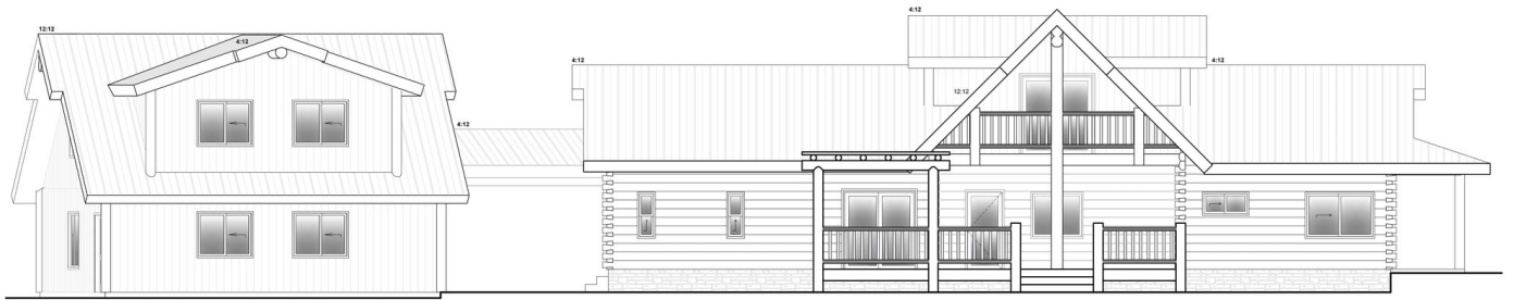
REAR ELEVATION
