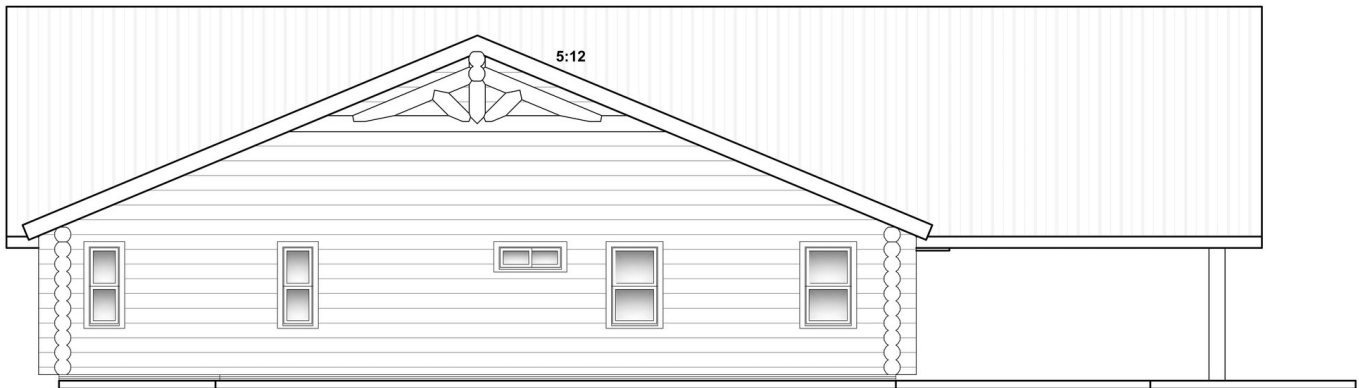
LEFT ELEVATION
