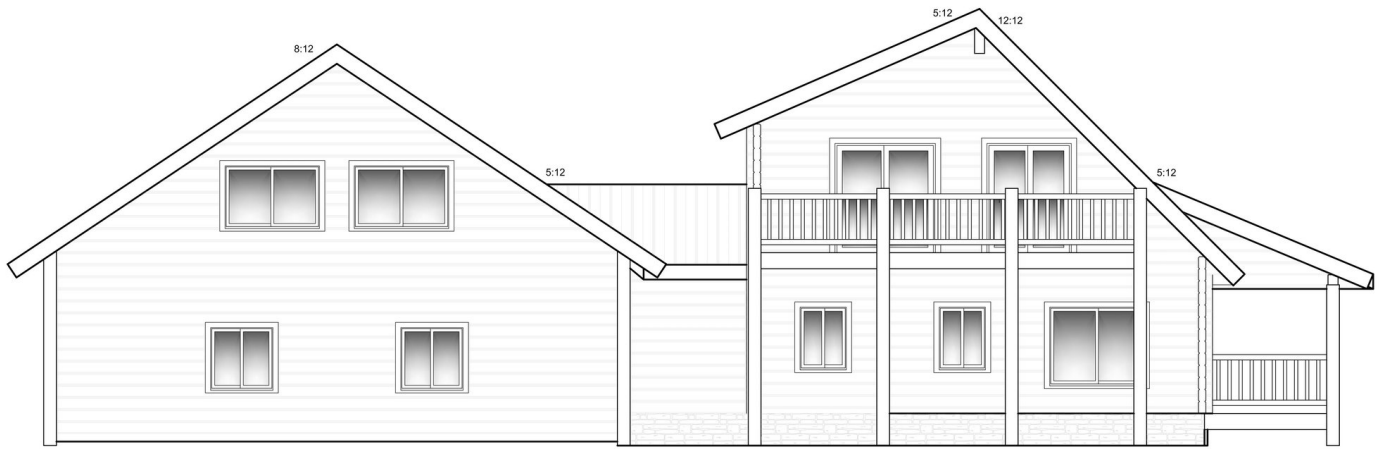
LEFT ELEVATION
