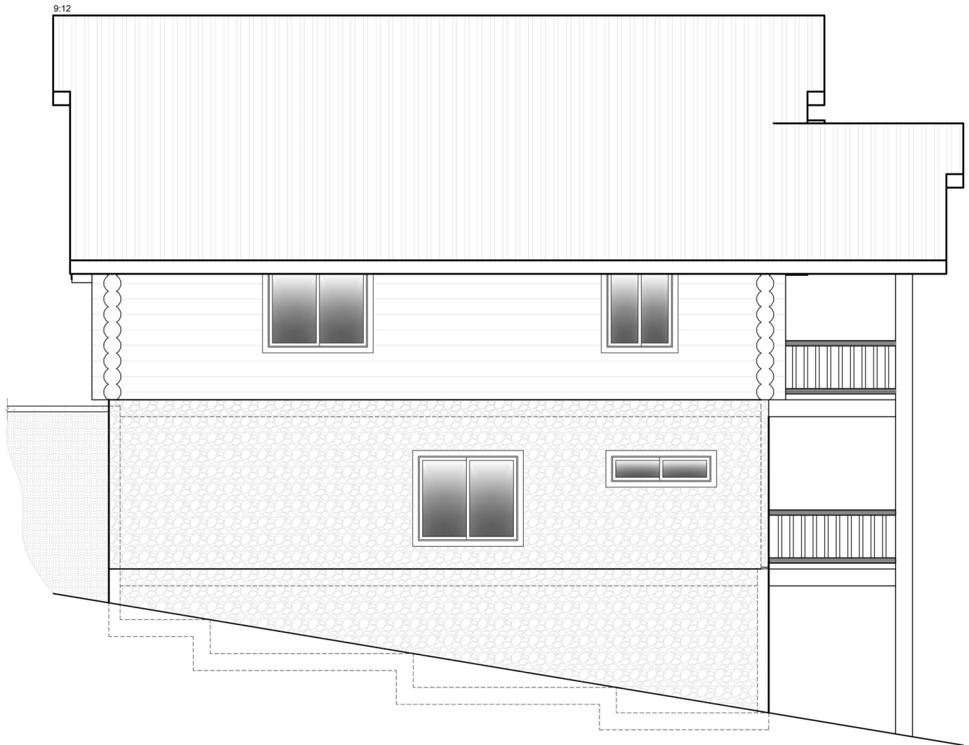
LEFT ELEVATION
